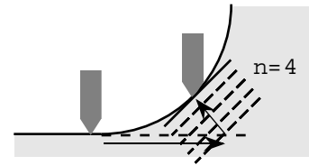
Figure 7: When a new plane equation would cause the probe to be embedded in the surface, the recovery time algorithm artificially lowers the plane to the probe position then raises it linearly to the correct position over n force loop cycles.
